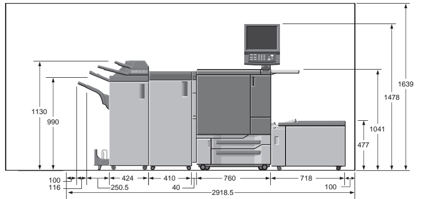
Front View bizhub PRESS C71hc + RU-516 + FS-612 + RU-509 + LU-202
