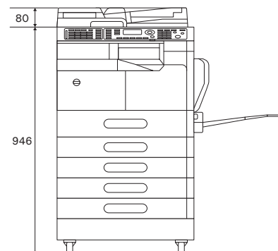
Front View bizhub 306/266 + DF-625 + PF-509 x4 + DK-708
