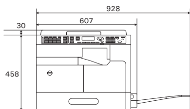
bizhub 226 (206) + OC-512
