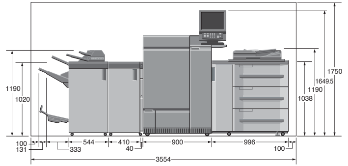
Front View bizhub PRESS C1100/C1085 + FS-532 (PI-502/MK-732/PK-522/SD-510) + RU-511 + RU-516 + Machine + WT-512 + PF-708
