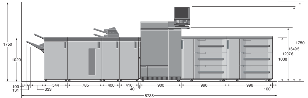
Front View bizhub PRESS C1100/C1085 + FS-532 + LS-506 + FD-503 + RU-511 + RU-516 + Machine + WT-512 + PF-707 + PF-707
