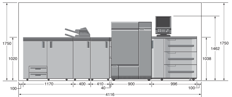
Front View bizhub PRESS C1100/C1085 + SD-506 + FD-503 + RU-511 + RU-516 + Machine + PF-707
