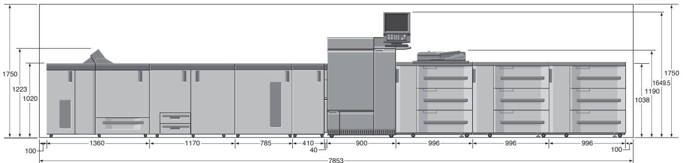
Front View bizhub PRESS C1100/C1085 + PB-503 + SD-506 + LS-506 + RU-511 + RU-516 + Machine + WT-512 + PF-708 + PF-707 + PF-707
