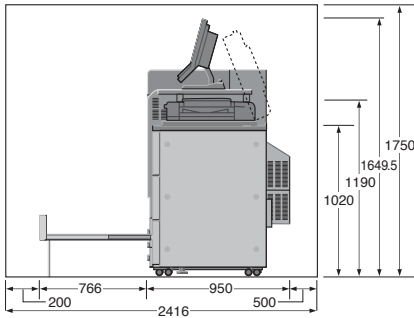
Side View bizhub PRESS C1100/C1085 + SD-506 + RU-511 + RU-516 + Machine + WT-512 + PF-708
